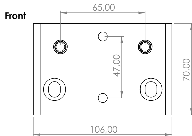
Eaglewing Adaptor
