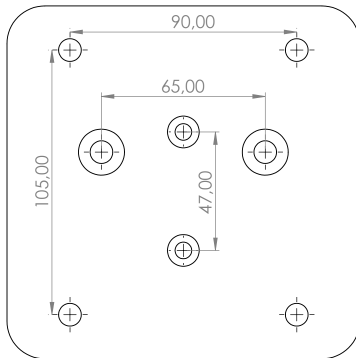
Eaglewing Adaptor
